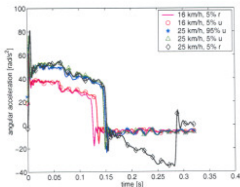
Figure 6: Sled pulse
