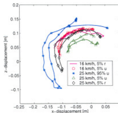
Figure 17 Trajectories of OC w.r.t. non rotating T1
