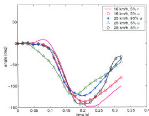
Figure 27: Head angle with respect to the sled
