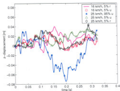
Figure 8: z-displacement of the occipital condyle with respect to T1
