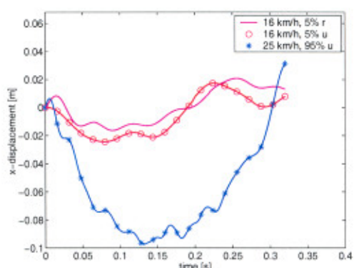
Figure 13: x -displacement of the pelvis anatomical origin with respect to the sled
