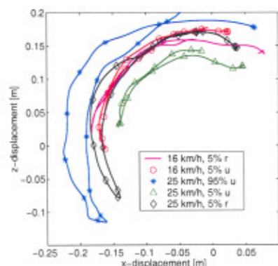
Figure 16 Trajectories of head CG w.r.t. non rotating T1
