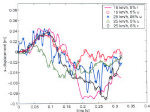
Figure 7: x-displacement of the occipital condyle with respect to T1
