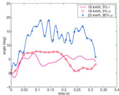
Figure 15: Pelvis angle with respect to the sled
