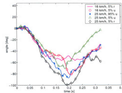
Figure 30: T1 angle with respect to the sled
